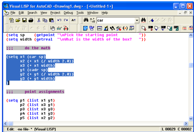
Figure 2.18 – Do the Math
