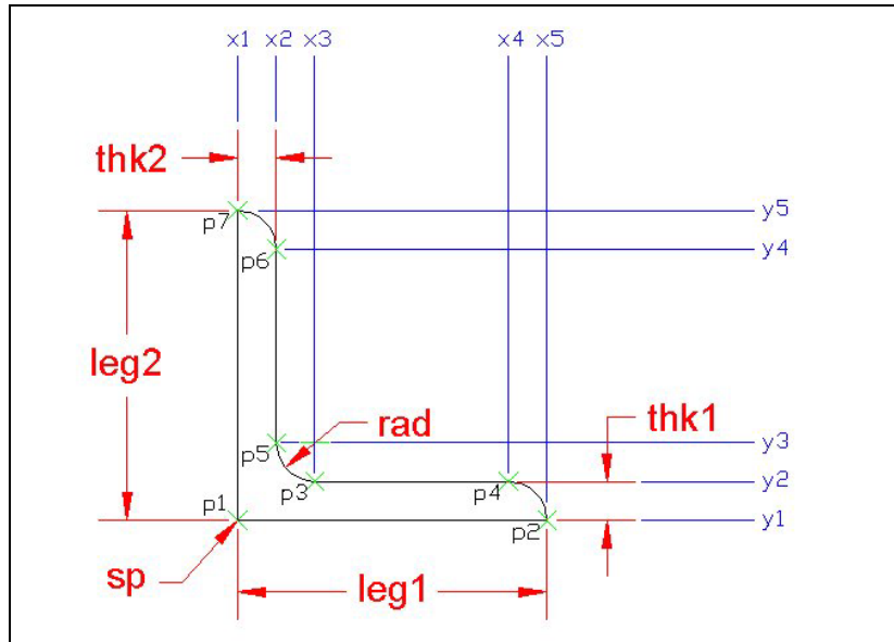
Figure 1.3 – The Anglemaker Problem
