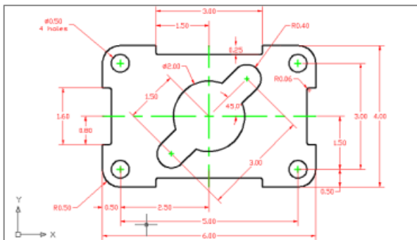
Figure 3.38 – Finished dimensioning the rectangular problem
