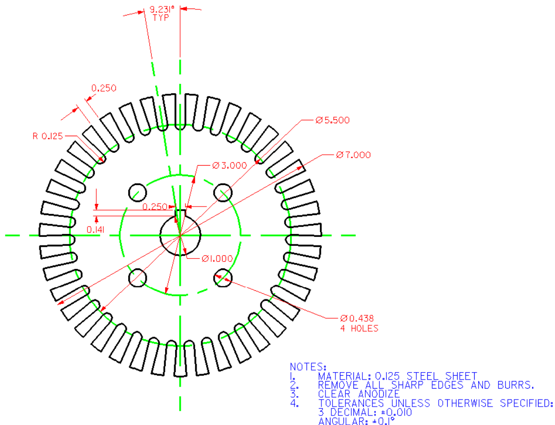
Figure B.1 – A Stamping
