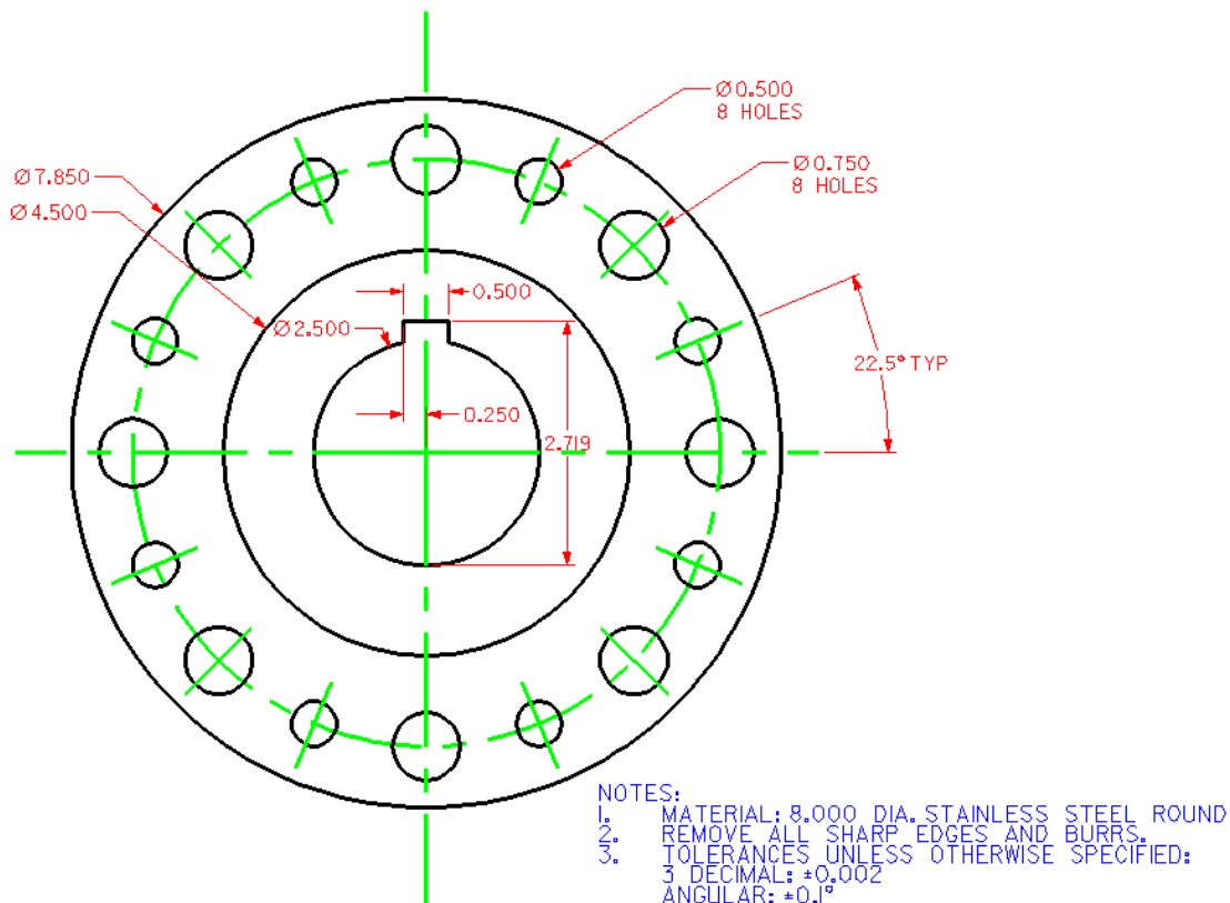
Figure B.2 – A Hub
