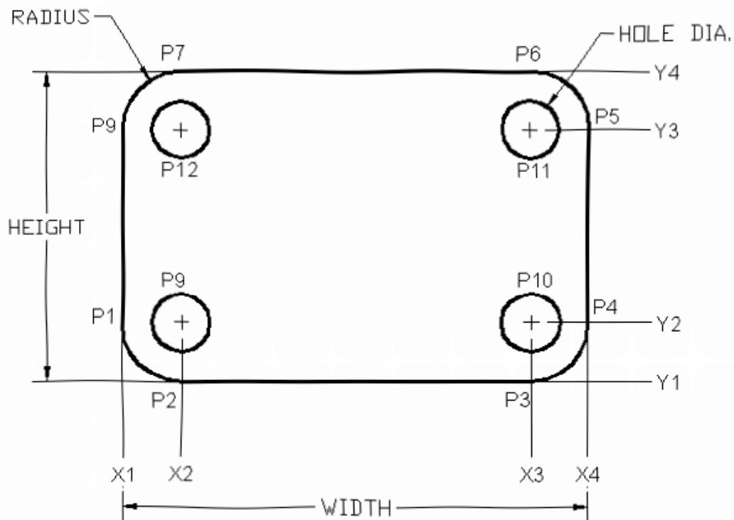
Figure 11.2 – Sketch of a Part Ready to Program
