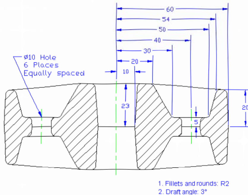
Figure 13.1 – Revolving Problem One Sketch
