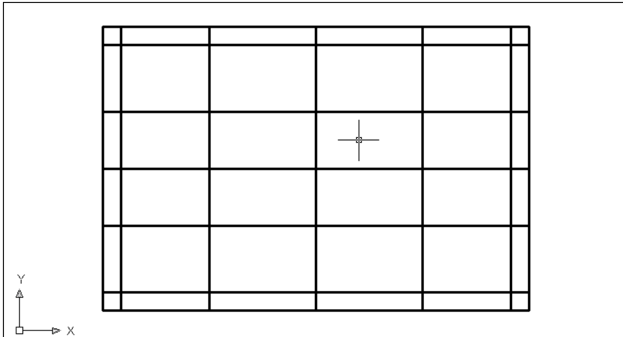
Figure 2.17 The 4 x 6 rectangle with two centerlines and eight offset lines
